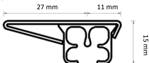
Smart Click top fix Bracket
