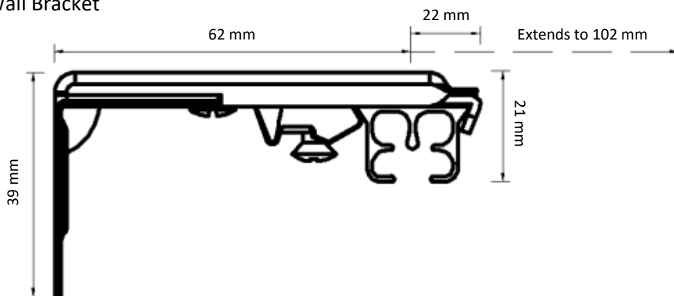
Double Adjustable Wall Bracket
