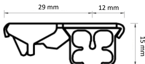
Spring Clip Top Fix Bracket with coverplate
