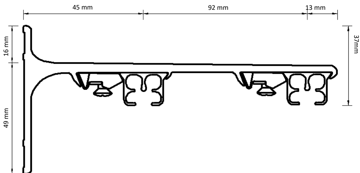
Slimline Double Bracket 15 cm
